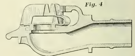
SECTIONAL VIEW OF DUST GUARD, CLOSED.
